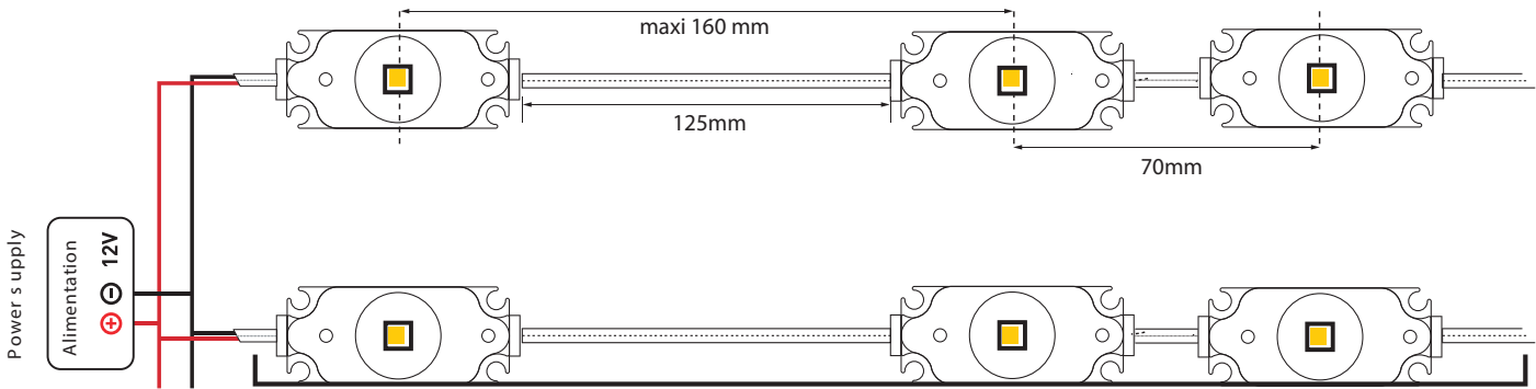
maximum 50 modules in series
